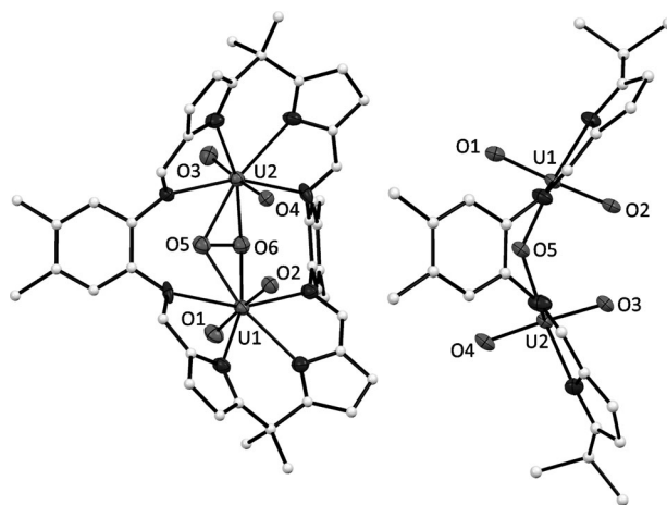
Figure 2. X-ray crystal structures of 3 (left) and 4 (right, side-on view). For clarity, all of the hydrogen atoms, K atoms, and solvent donors are omitted. Where shown, ellipsoids are set at 50 % probability.
